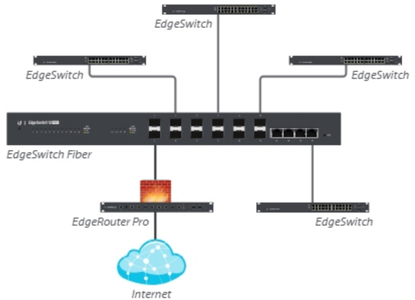
Multiple EdgeSwitches connect to the EdgeSwitch Fiber, which has an SFP uplink to the Ubiquiti® EdgeRouter™ Pro.
